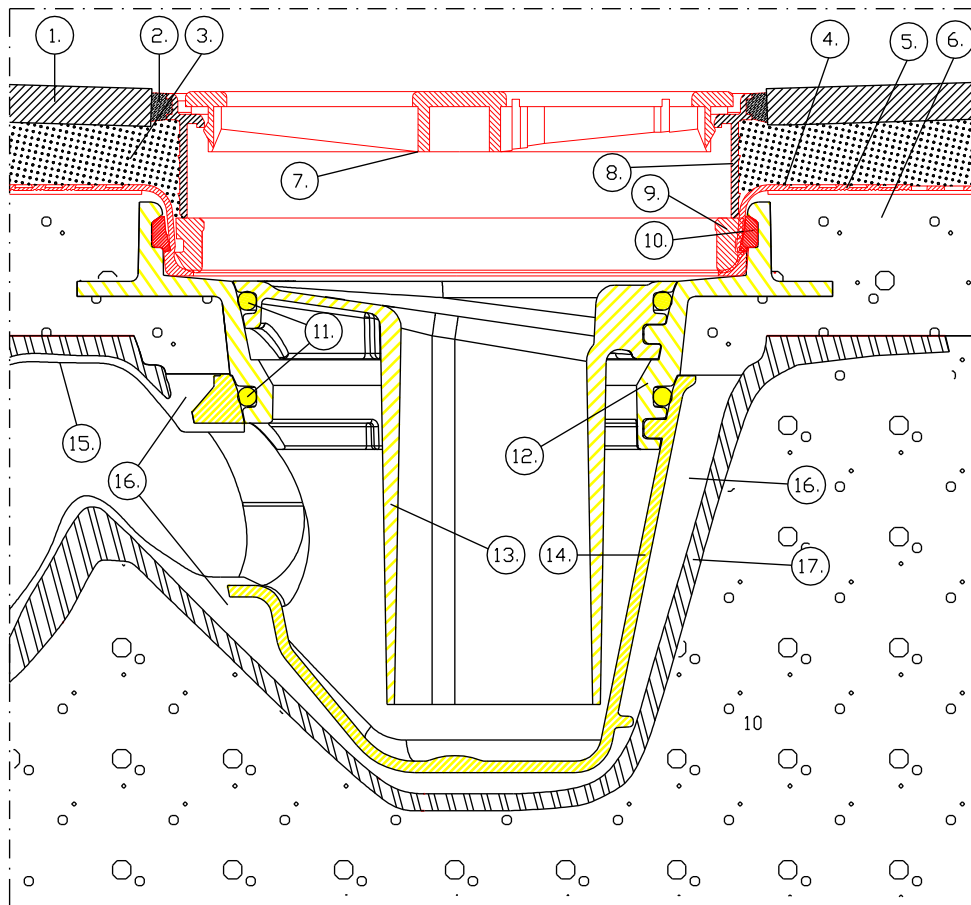
PRINCIPLE SKETCH 1:2
